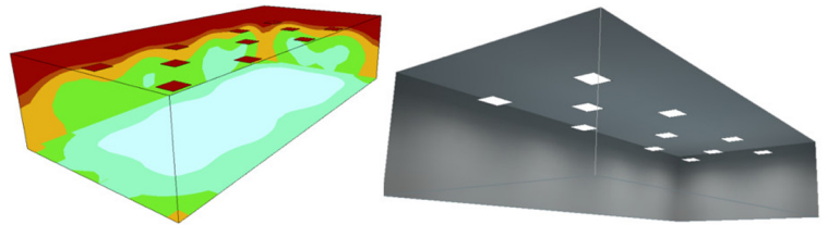
Lighting designs showing light distribution when using 600x600 LED panels
