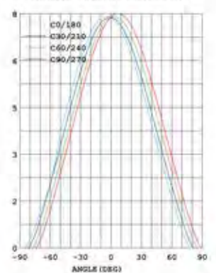
LUMINOUS INTENSITY DISTRIBUTION
