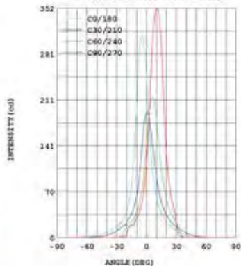
LUMINOUS INTENSITY DISTRIBUTION
